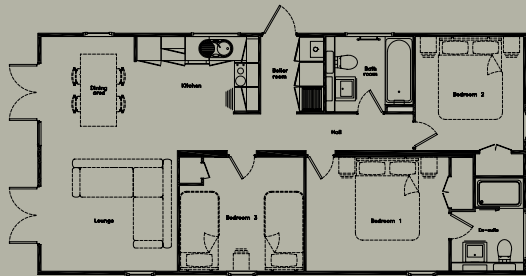
Overall size: 40 x 20ft 3 Bed Gross Internal Area: 791sqft (73.44sq/m)
