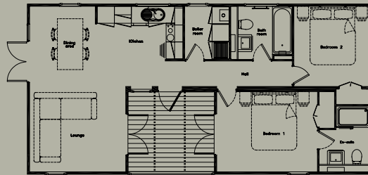
Overall size: 40 x 20ft 2 Bed with conservatory Gross Internal Area: 695sqft (64.54sq/m)
